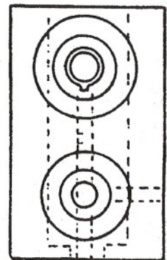
8 9 RETAINER SET SCREW 8-32 THD, 5/64 L-WRENCH
